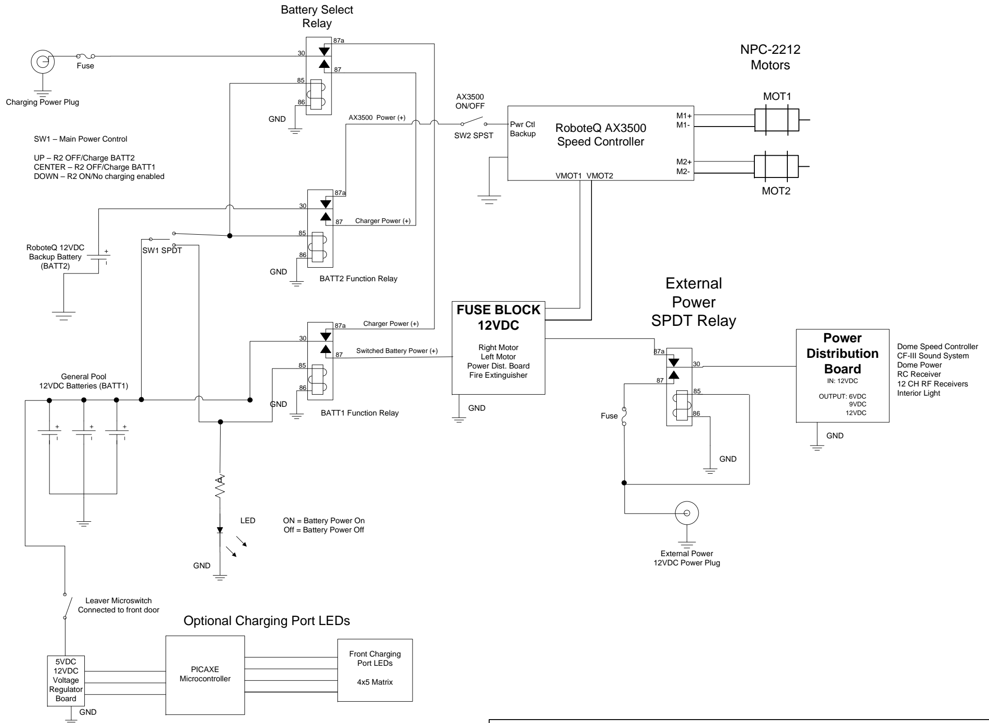
R2-D2 12VDC Overview Wiring with Battery Charging System and External Power
